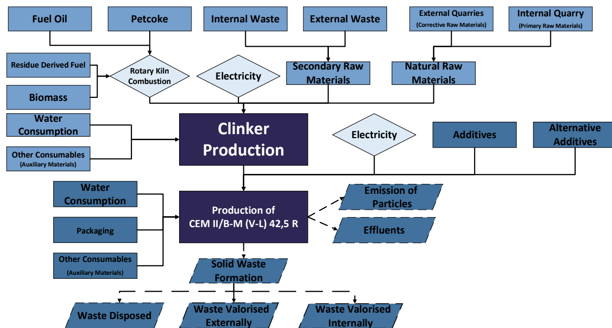
Figure 1: Simplified flowchart for CEM II/B-M (V-L) 42,5 R cement production inventory.
